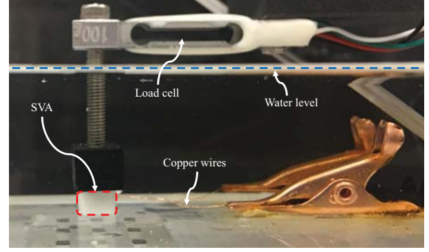
Fig. 2. Experimental setup that uses a load cell to measure the force applied by an SVA.
