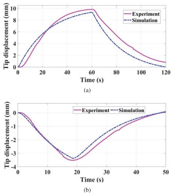
Fig. 8. Simulated and measured robot tip displacement along the x -axis when (a) SVA numbers 1 to 8 are actuated with a square wave of amplitude 1.8 V applied for 60 seconds; (b) SVA numbers 4, 9, and 15 are actuated with a square wave of amplitude 3.6 V for 15 seconds (Case 8, Table II).
