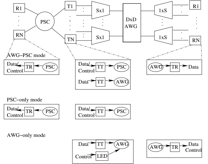
Fig. 3. Detailed node architecture
