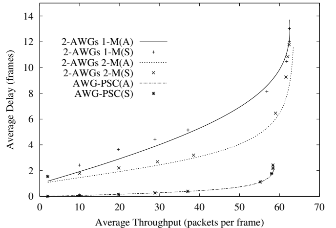
Fig. 12. Throughput–delay performance comparison for three networks: D –buffered AWG||AWG with one control, D –buffered AWG||AWG with two controls, and AWG||PSC
