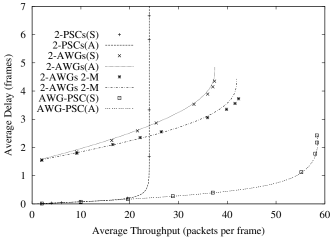
Fig. 11. Throughput–delay performance comparison for three networks: PSC||PSC, AWG||AWG, and AWG||PSC
