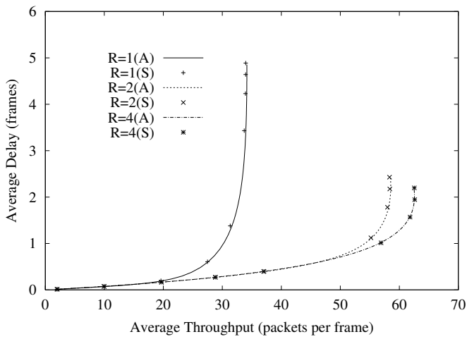
Fig. 8. Throughput–delay performance for R = 1, 2, and 4 used FSRs. ( D = 4 , fixed)
