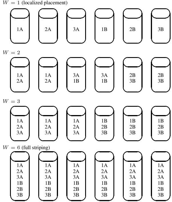
Fig. 1. Group striping of M = 3 movies (denoted by 1, 2, and 3) over D = 6 disks with striping widths of W = 1, 2, 3 , and 6. We use uniform replication in this example; thus there are D/M = 2 copies (denoted by A and B) of each movie stored in the disk array.
