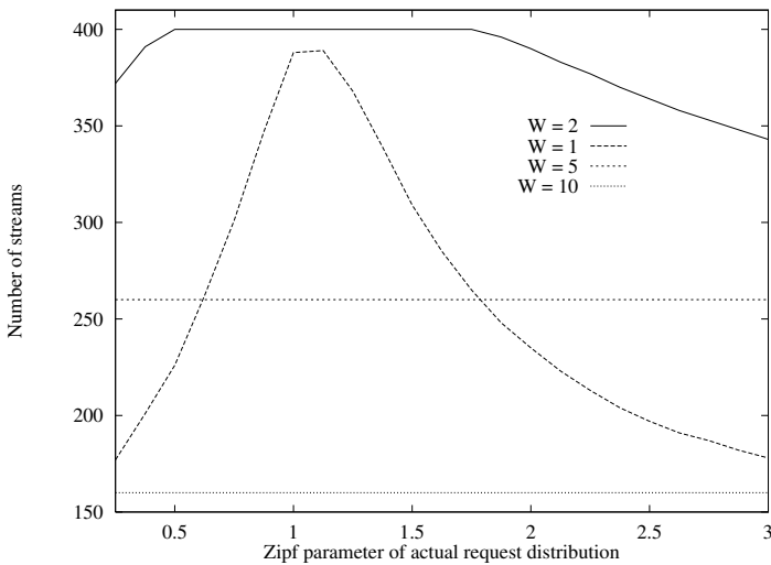
Fig. 2. Number of streams as a function of the Zipf parameter \xi of the actual user request distribution. The movies are replicated according to the expected user request distribution, which is assumed to be the Zipf distribution with parameter \xi = 1 .
